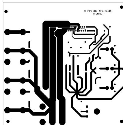
Figure 48. Bottom Layer
