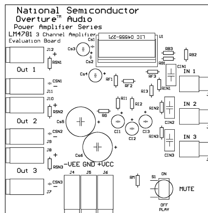
Figure 46. Silk Layer
